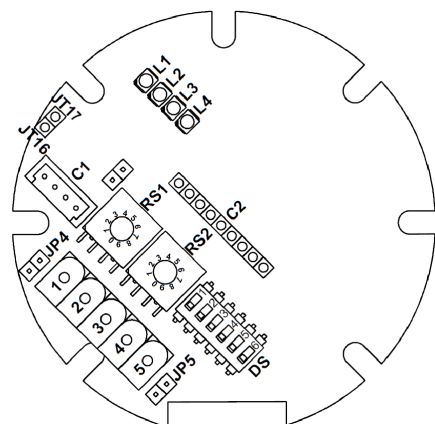
Fig. 5: Internal disposition
