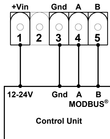
Fig. 7: Example of Modbus® connection.
